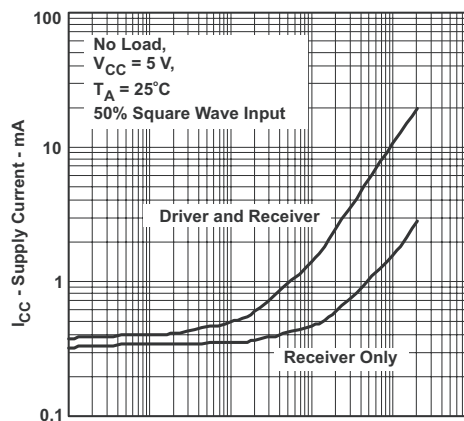
图 6-4. SN65HVD3088E RMS Supply Current versus Signal Rate
